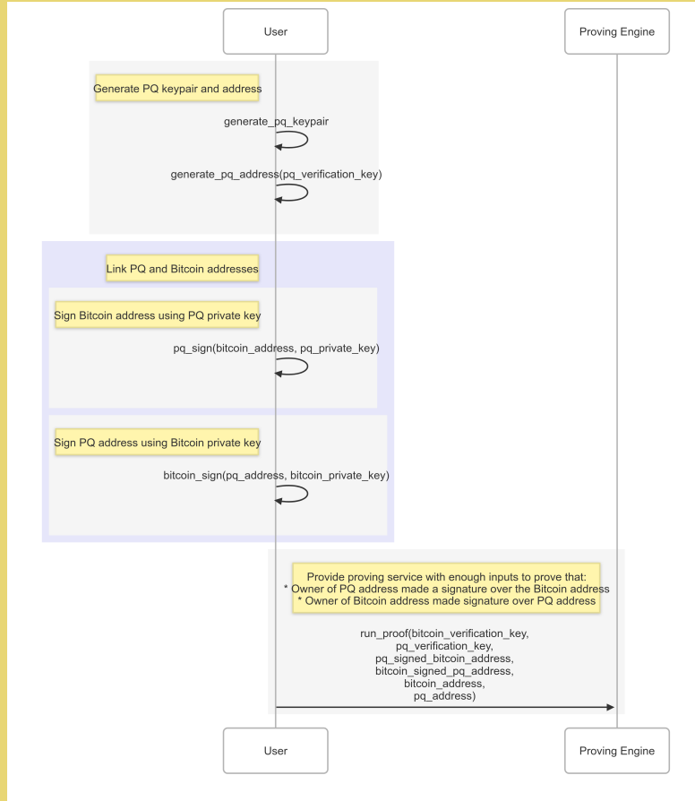
Figure 2: Detailed view of the User's cryptographic steps, highlighting secure PQ key generation, mutual cross-signing of addresses, and preparation of verification data for the Proving Engine
