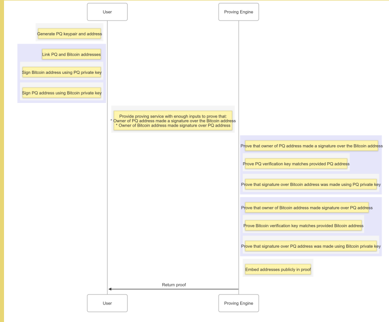
Figure 1: Overview of the cryptographic linkage process, illustrating high-level interactions between the User and the Proving Engine to securely associate Bitcoin addresses with quantum-resistant (PQ) addresses.
