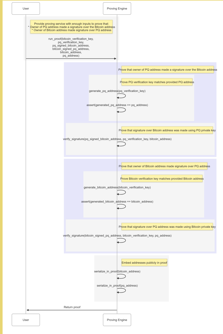
Figure 3: In-depth process of the Proving Engine’s validation steps, demonstrating rigorous cryptographic verification and the creation of a publicly verifiable proof embedding both addresses securely.
